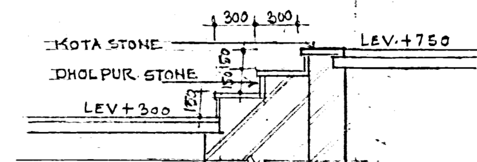
SECTION AT XX'
